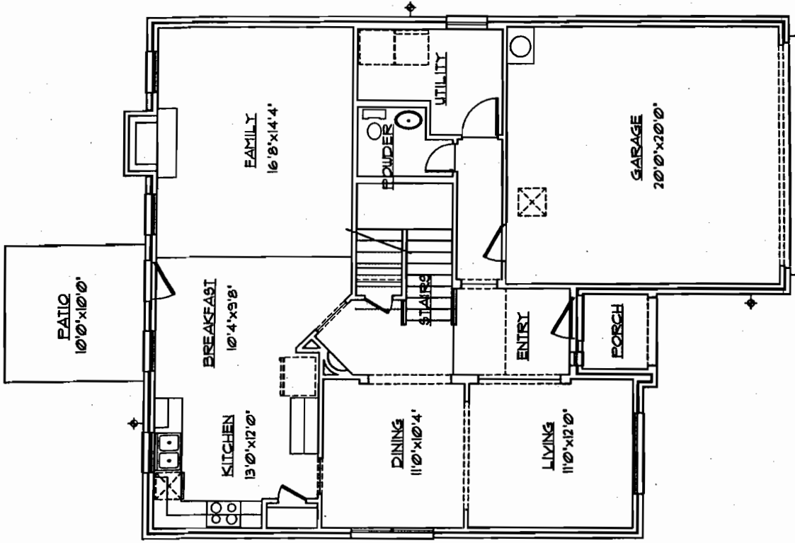
FIRST FLOOR PLAN 1"=10'0" 2408 SQ. FT. MJW#01181KEY
