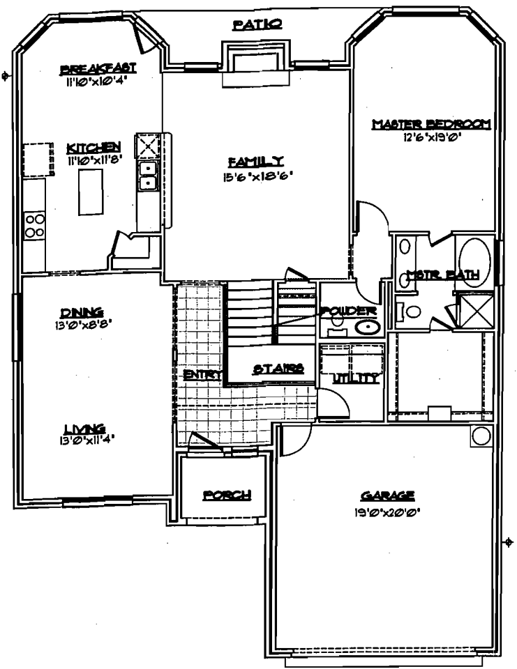
FIRST FLOOR PLAN NTB
