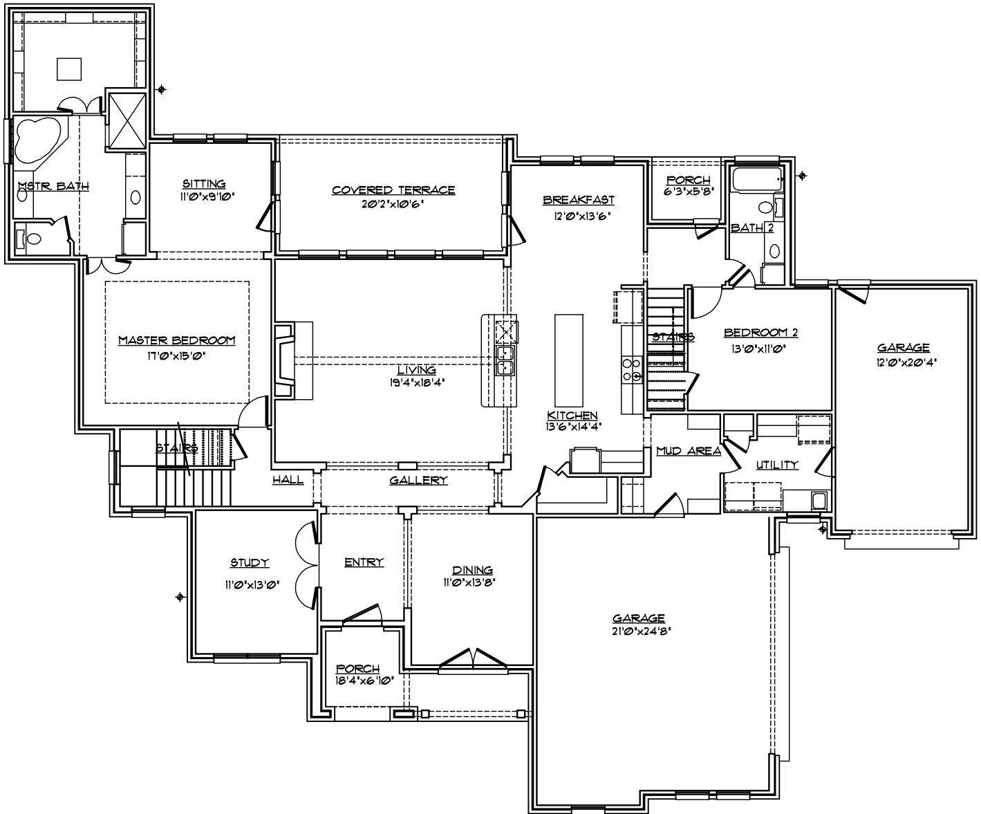
ARAPAHO - FIRST FLOOR PLAN 5 BEDROOM / 4 BATH (2884#+236#OPT.MEDIA) 05037
