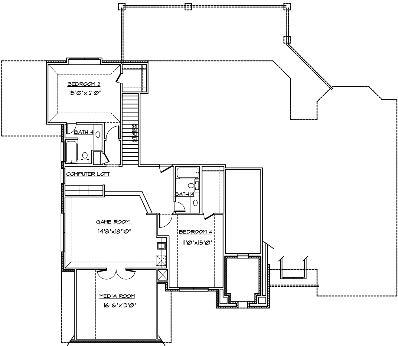
ASPEN - SECOND FLOOR PLAN
