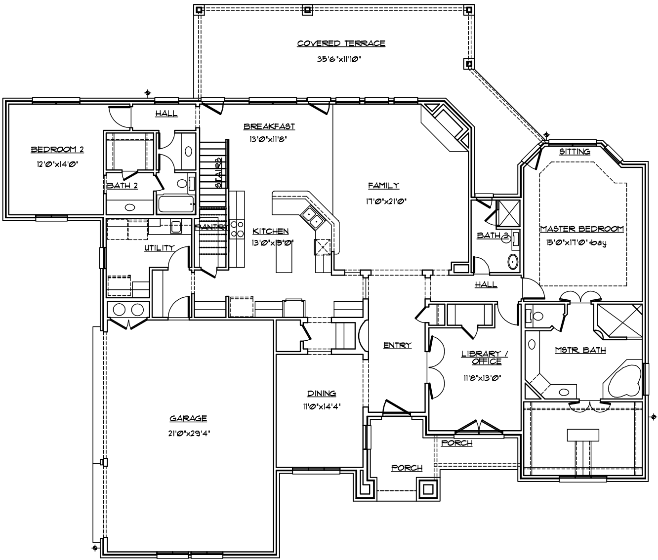
ASPEN - FIRST FLOOR PLAN 5 BEDROOM - 5 BATH (OPT.MEDIA) 4172# 07001
