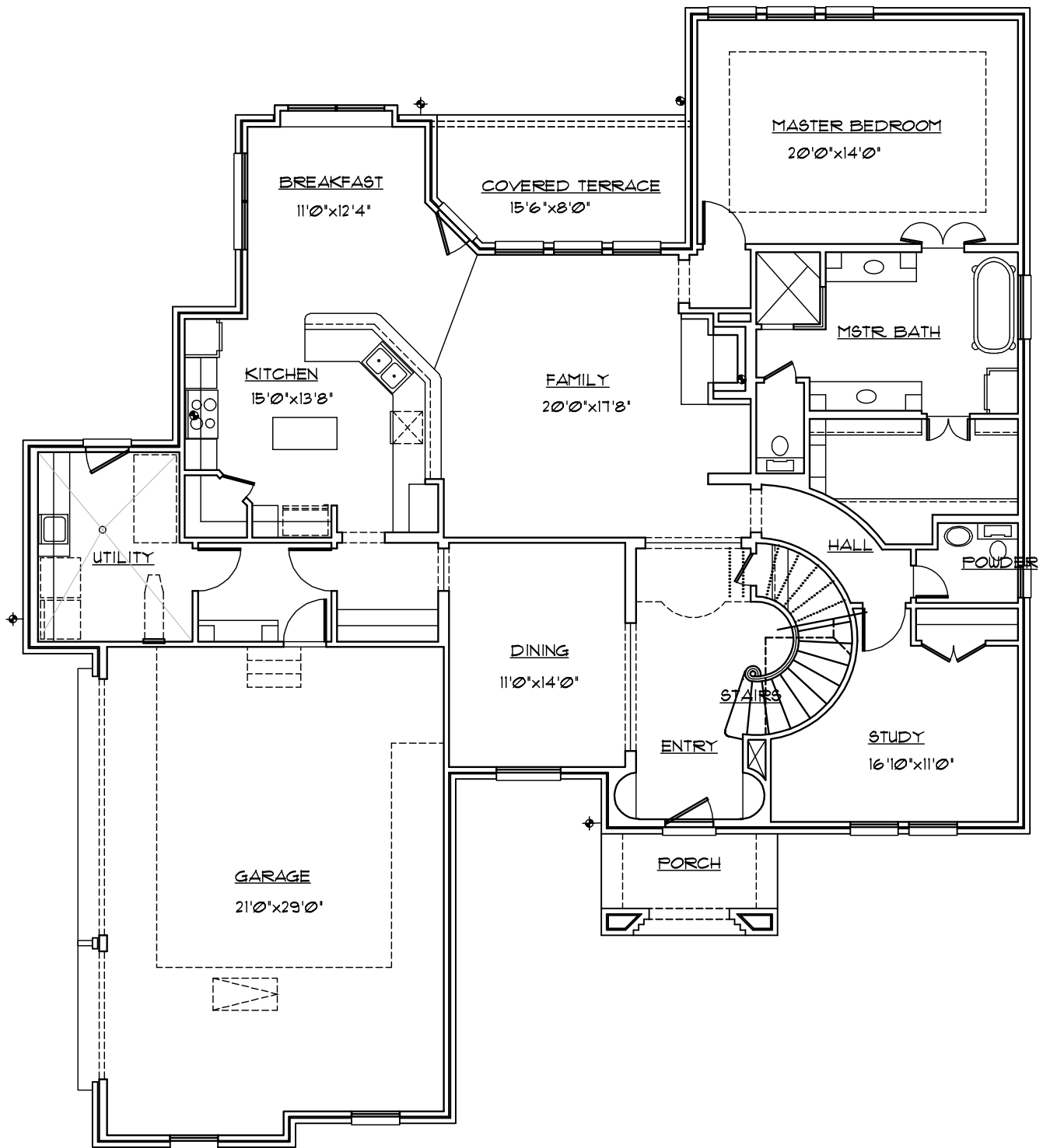
BRECKENRIDGE - FIRST FLOOR PLAN 4 BEDROOM / 3.5 BATH (3190) 06057
