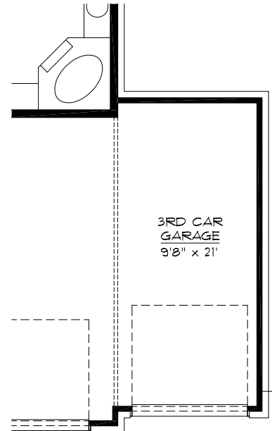
OPTIONAL 3RD CAR GARAGE
