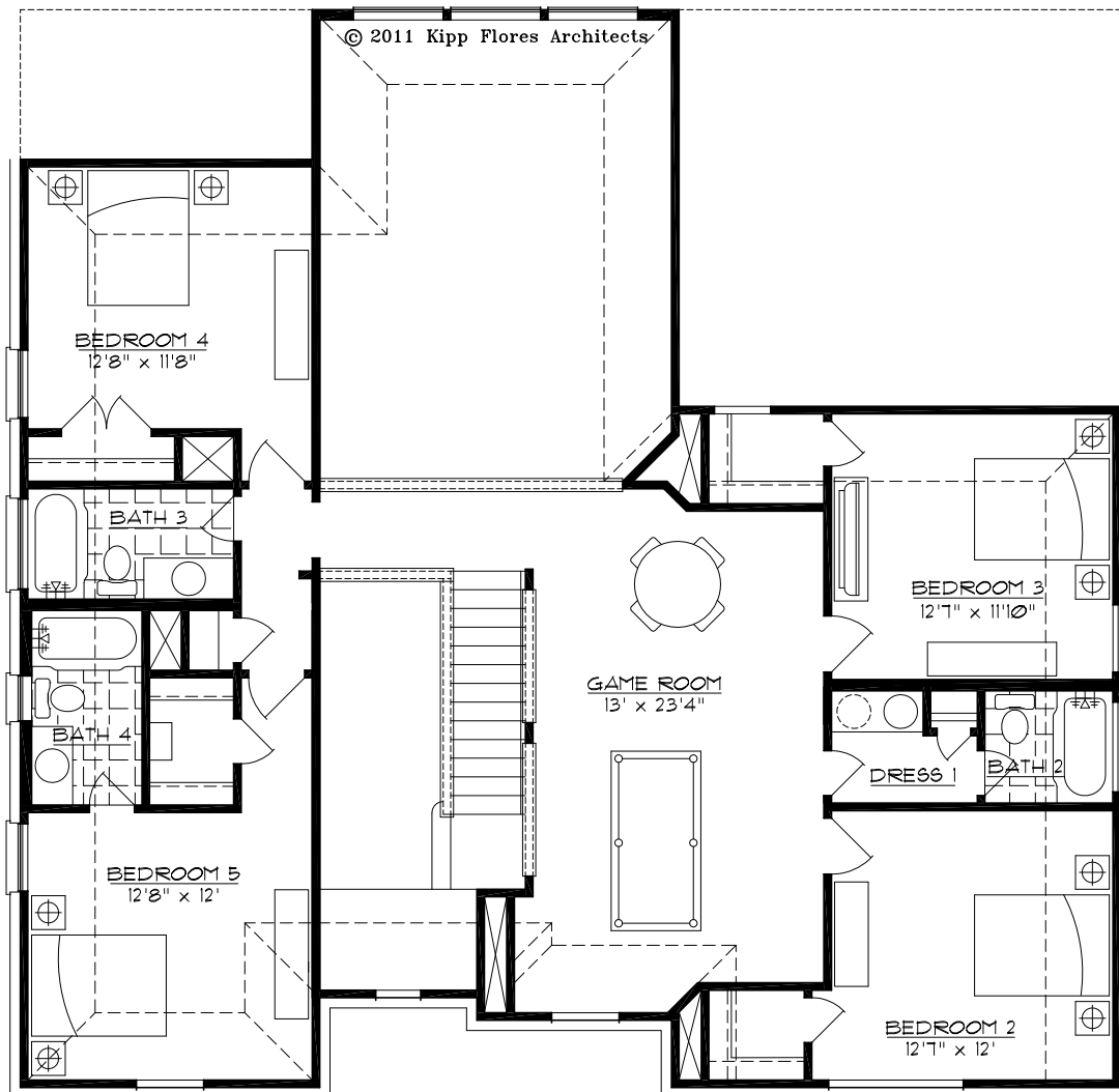
OPTIONAL 2ND FLOOR PLAN (BEDROOM 5/ BATH 4) 295 SQ. FT (with 1st & 2nd floor = 3376 SQ. FT.)
