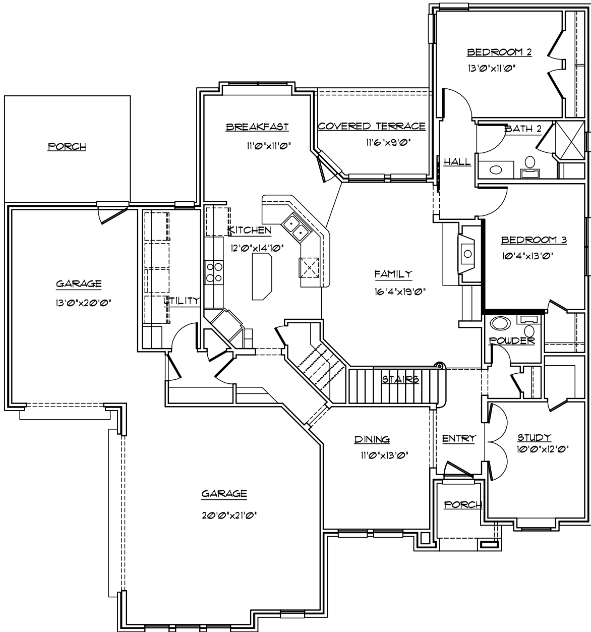
TELLURIDE - FIRST FLOOR PLAN 3 BEDROOM / 3.5 BATH (2676#+OPT.331#MEDIA) 06031
