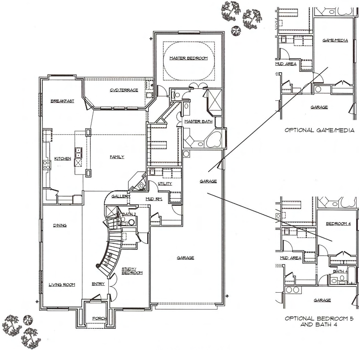
FIRST FLOOR PLAN 'A'
