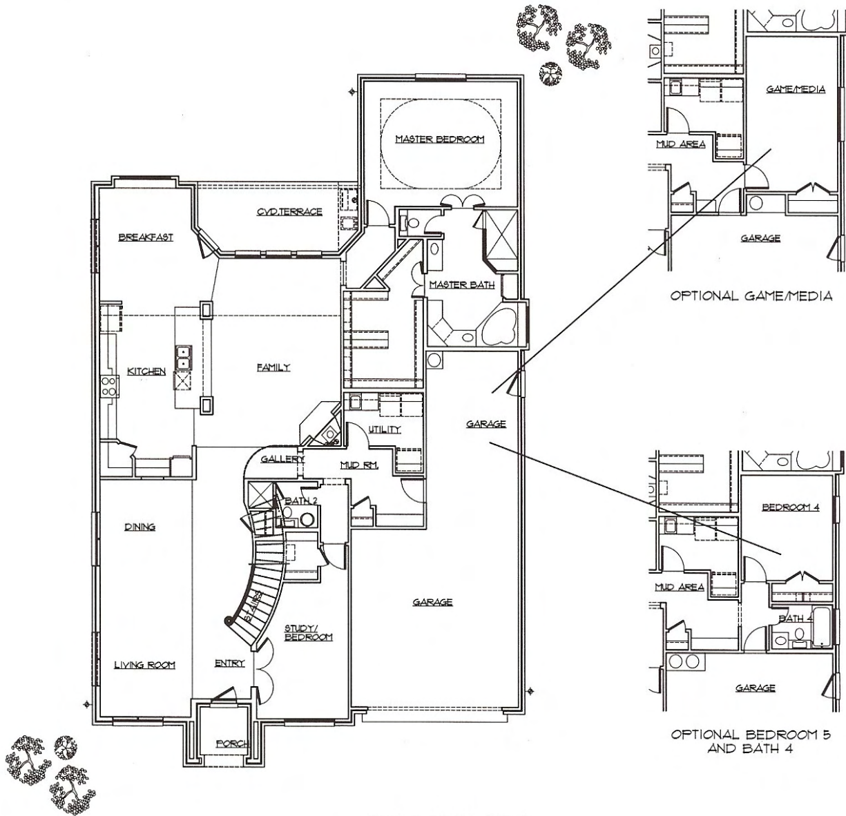
FIRST FLOOR PLAN 'B'
