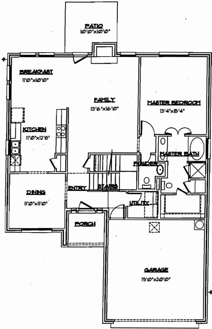
FIRST FLOOR PLAN 'A' NT6
