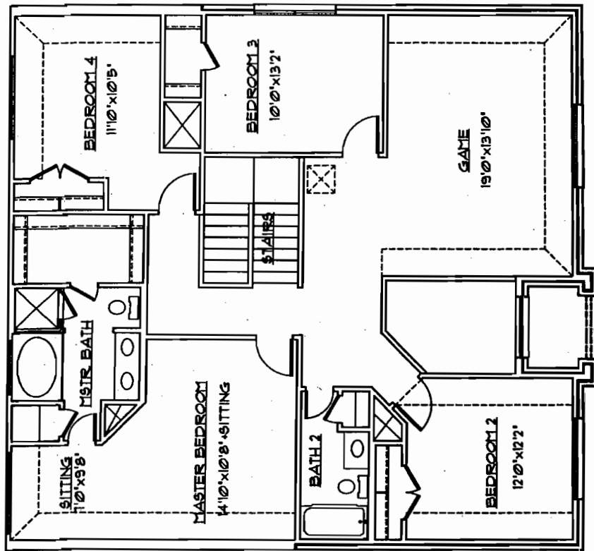
SECOND FLOOR PLAN 1"=10'0"
