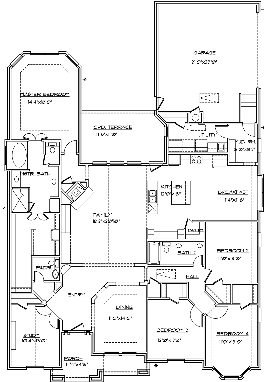
MONARCH - FLOOR PLAN 4 BEDROOM / 2.5 BATH (2828#) 06078
